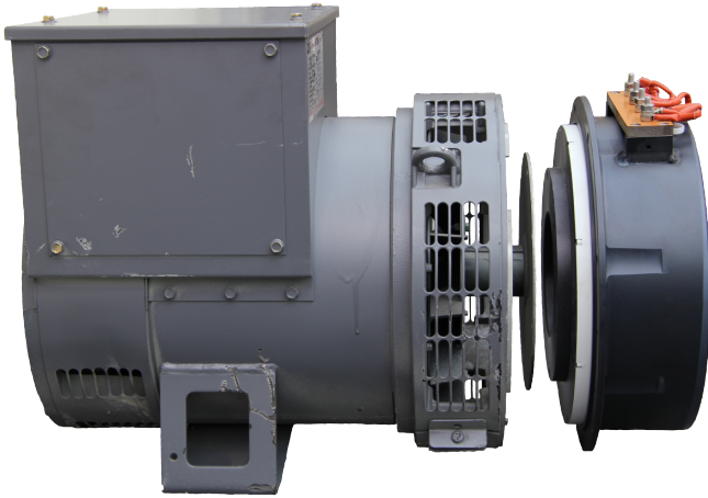
Figure 1, a Leroy Somer Alternator rated at 20 kVA (16 kW), popularly used by Caterpillar and other major AC Generator producers, next to the Polar model 8220 “DC” alternator, rated at 16 to 22 kW (depending on RPM).
