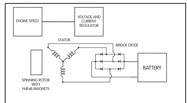
DC alternator
