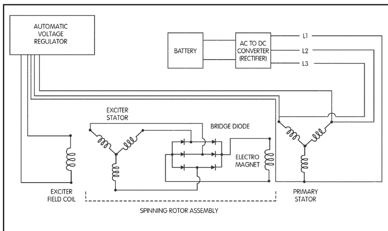
AC alternator
